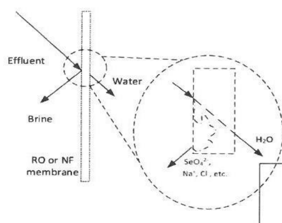
Fig. 1 Process of membrane separation: reverse osmosis (RO) and nanofiltration (NF)
